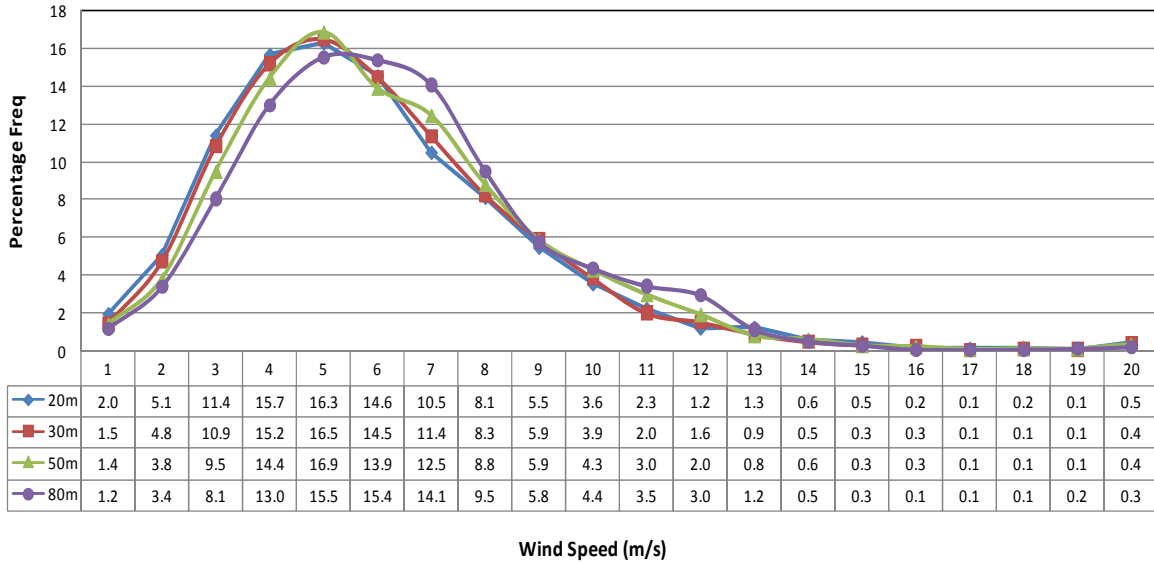
Percentage Wind Frequency Distribution at Kallar Kahar (June-2009)
