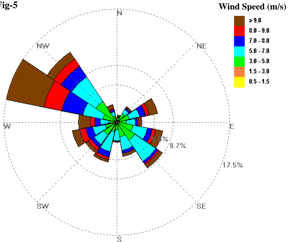
Wind Rose at Kallar Kahar (50m height during 01 month)
