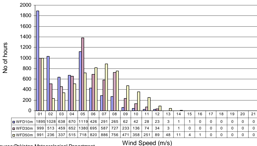
Wind Frequency Distribution at Karachi (Mar to May) in three years
