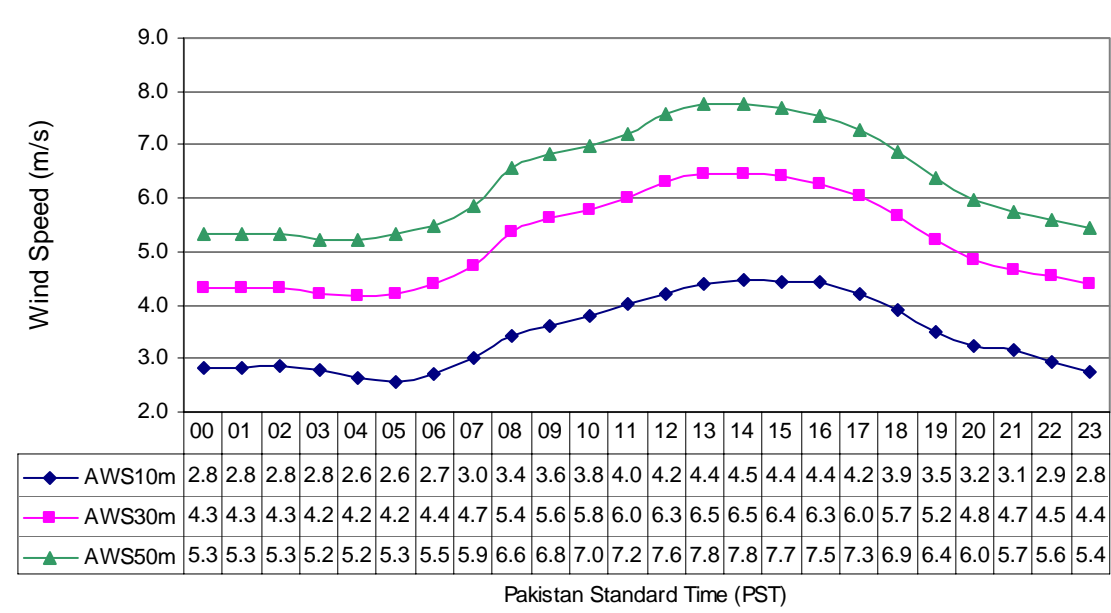
Diurnal Variation of Wind Speed at Karachi (Jun to Aug) in three Years
