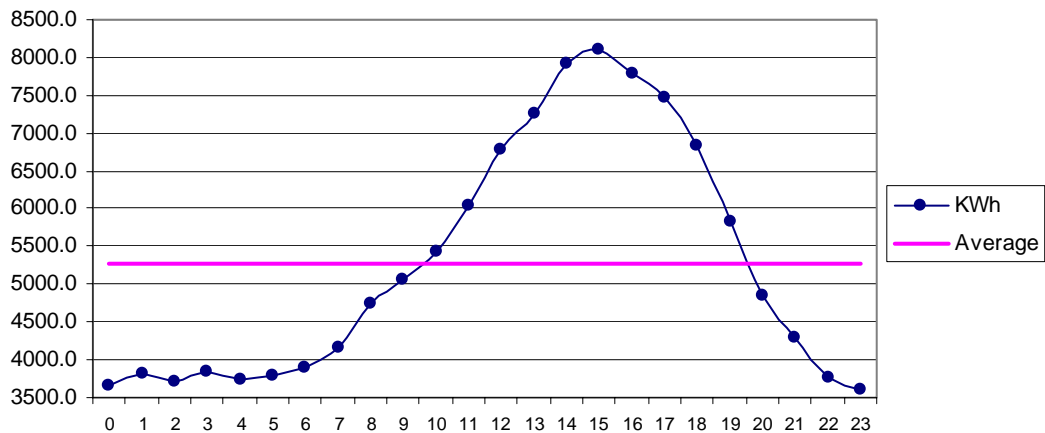
Fig 29 HawksBay Jun: Diurnal Variation of Wind Genrated Electric Energy Output
