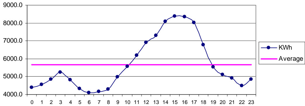
Fig 28 HawksBay May: Diurnal Variation of Wind Genrated Electric Energy Output
