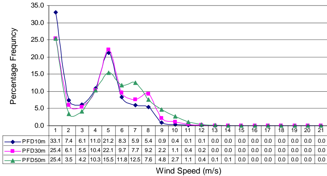
Percentage Wind Frequency Distribution at HawksBay (Sep to Nov) in three years
