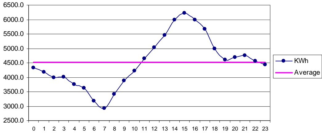
Fig 27 HawksBay Apr: Diurnal Variation of Wind Genrated Electric Energy Output
