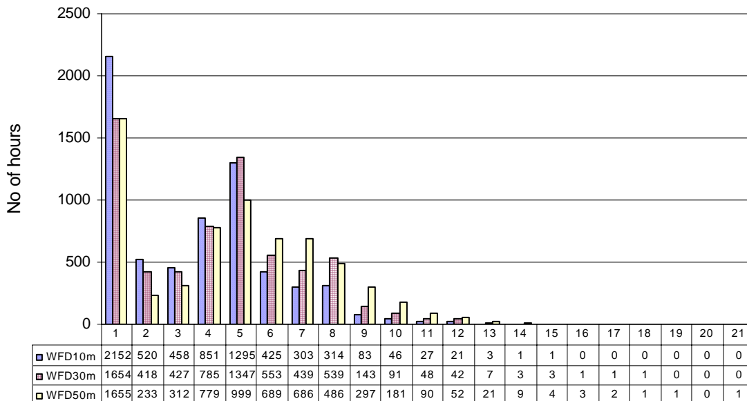
Wind Frequency Distribution at HawksBay (Dec to Feb) in three years
