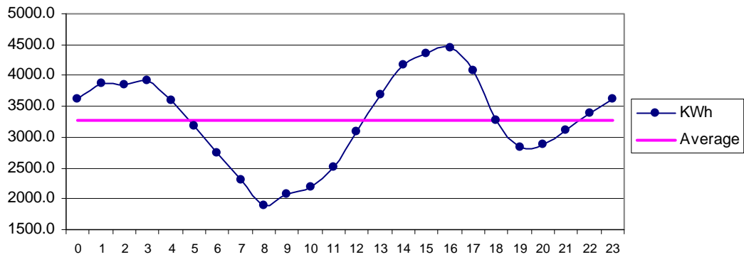
Fig 26 HawksBay Mar: Diurnal Variation of Wind Genrated Electric Energy Output
