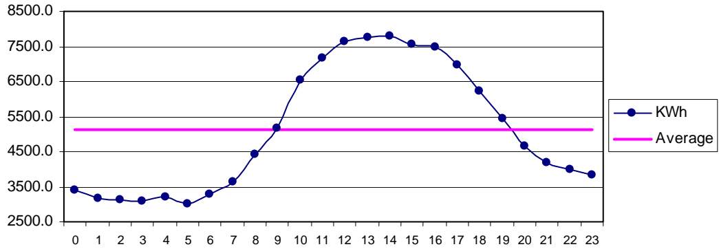
Fig 30 HawksBay July: Diurnal Variation of Wind Genrated Electric Energy Output
