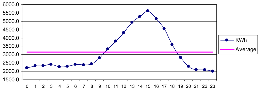
Fig 32 HawksBay Sep: Diurnal Variation of Wind Genrated Electric Energy Output
