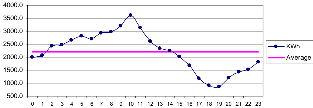
Fig 24 HawksBay Jan: Diurnal Variation of Wind Genrated Electric Energy Output
