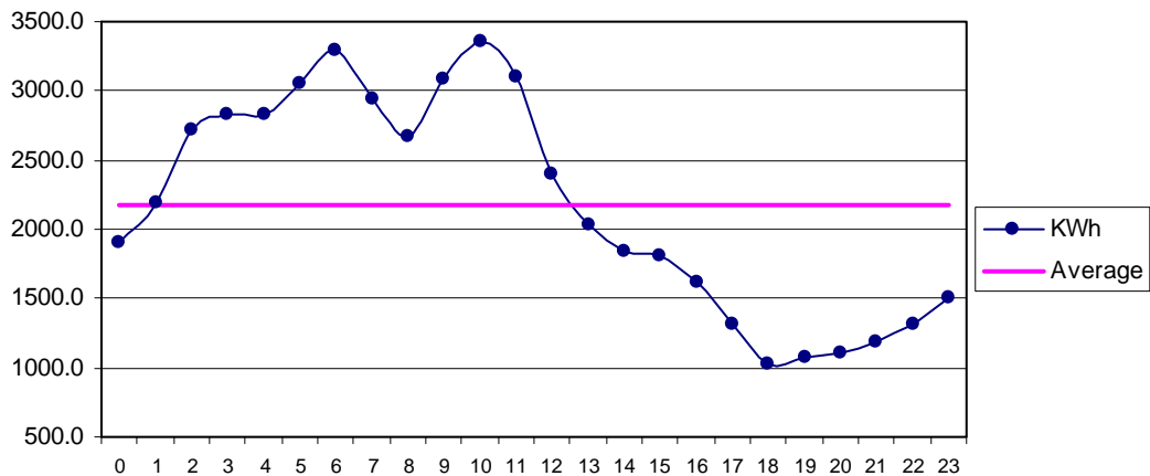
Fig 35 HawksBay Dec: Diurnal Variation of Wind Genrated Electric Energy Output
