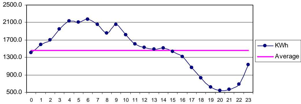
Fig 34 HawksBay Nov: Diurnal Variation of Wind Genrated Electric Energy Output
