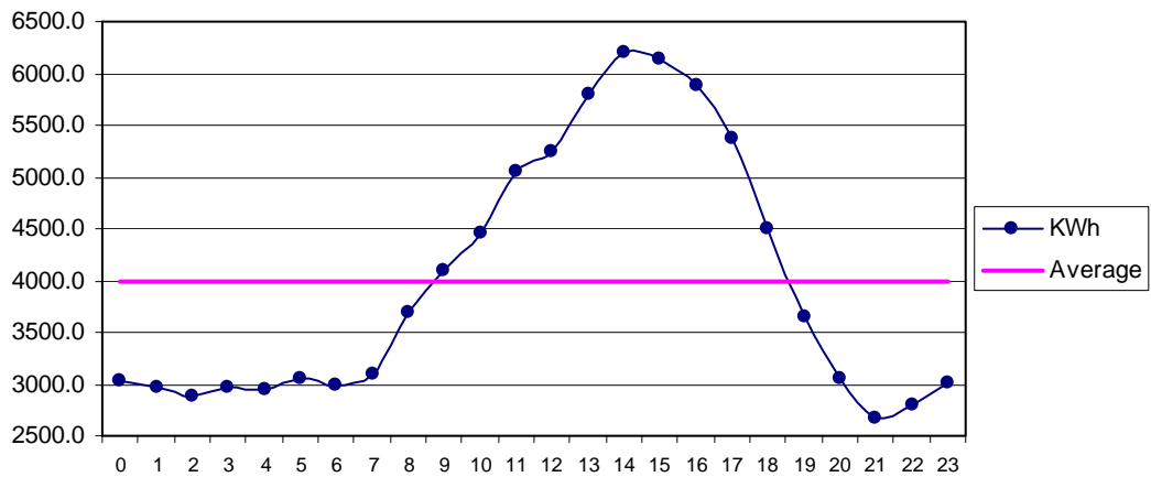
Fig 31 HawksBay Aug: Diurnal Variation of Wind Genrated Electric Energy Output
