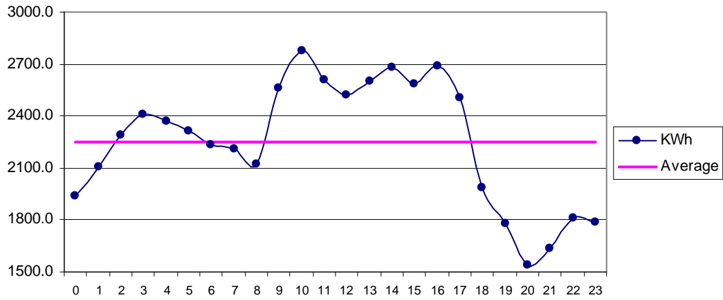
Fig 25 HawksBay Feb: Diurnal Variation of Wind Genrated Electric Energy Output
