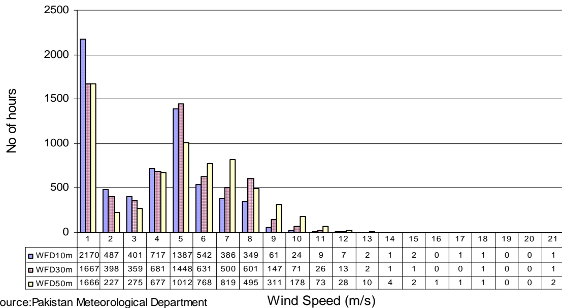
Wind Frequency Distribution at HawksBay (Sep to Nov) in three years
