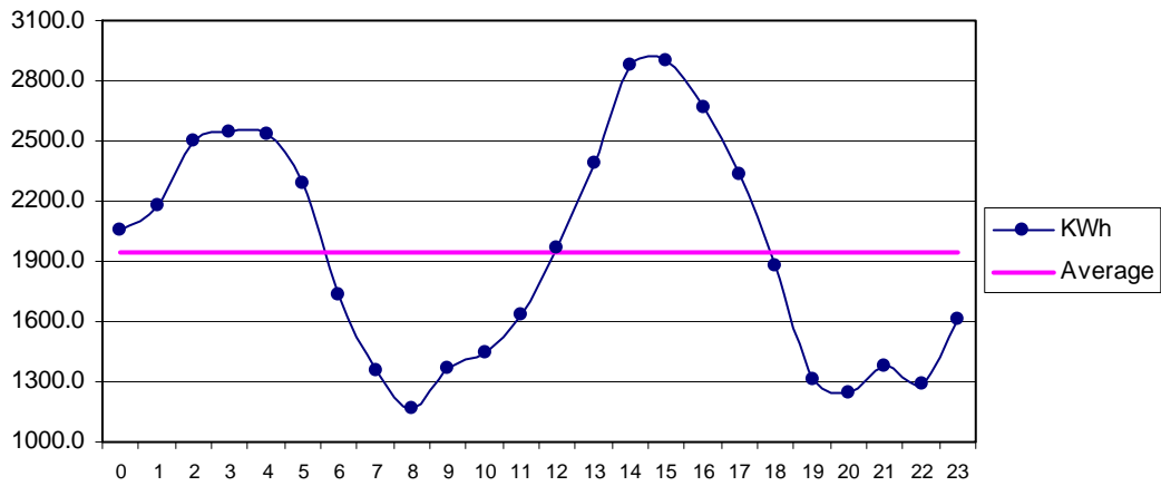
Fig 33 HawksBay Oct: Diurnal Variation of Wind Genrated Electric Energy Output
